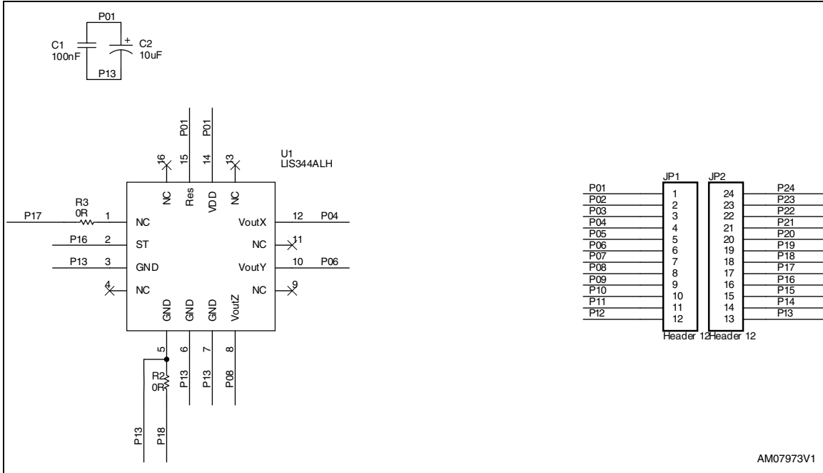
Figure 1. Schematic and connection diagram
