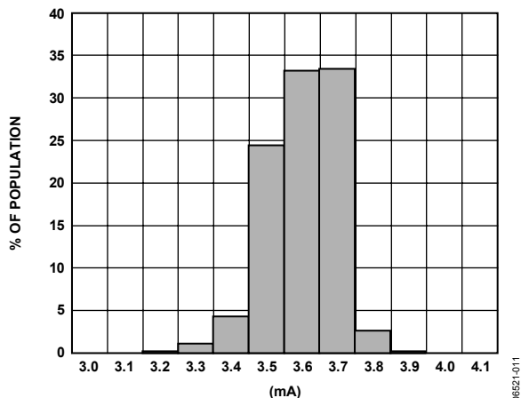
Figure 12. Current Consumption at 25°C ( V_{RATIO} = 5 V )
