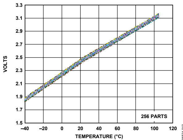
Figure 14. V_{TEMP} Output over Temperature, 256 Parts ( V_{RATIO} = 5 V )
