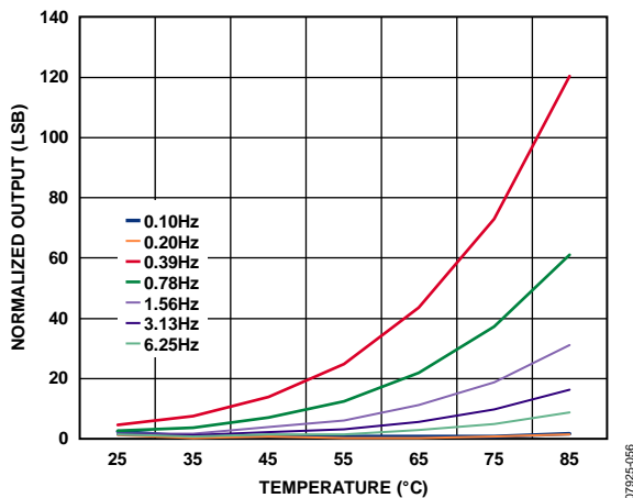
Figure 53. Typical X-Axis Output vs. Temperature at Lower Data Rates, 07925-056
