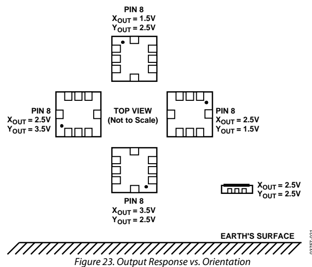
Figure 23. Output Response vs. Orientation
