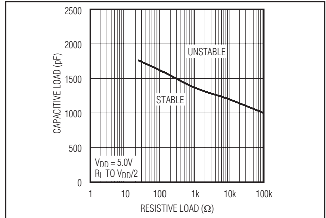
Figure 6. Capacitive-Load Stability
