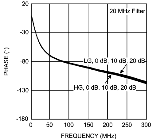
Phase vs. Gain
