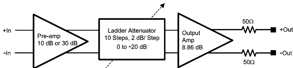
FIGURE 1. LMH6518 Signal Path Block Diagram
