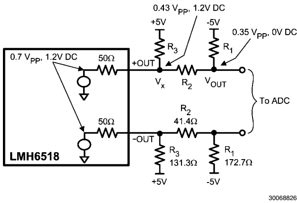
FIGURE 5. Output CM Shift Scheme
