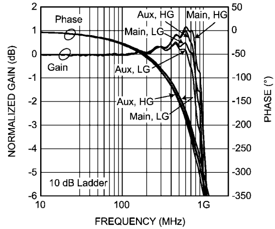
Main vs. Auxiliary Response
