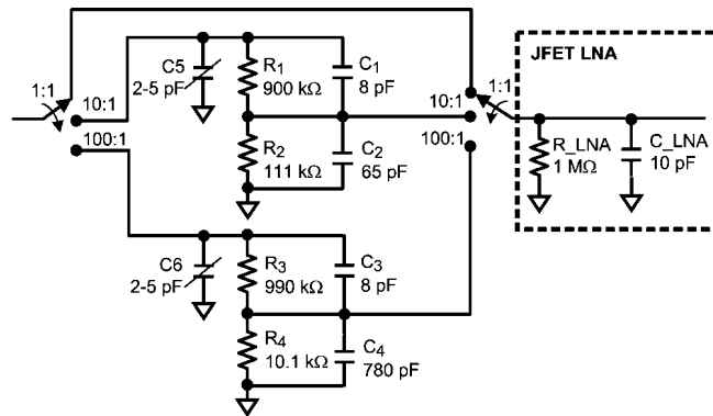
FIGURE 15. Front End Attenuator for Figure 13 JFET LNA
