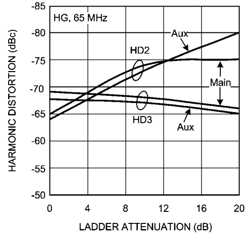
Main and Auxiliary Distortion Comparison
