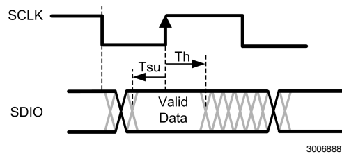
FIGURE 11. Write Timing
