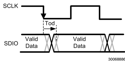
FIGURE 10. Read Timing
