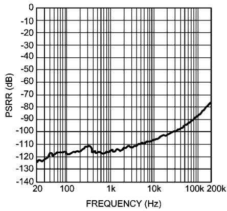
PSRR+ vs Frequency V_{CC} = 12V, V_{EE} = -12V R_L = 600\Omega, f = 200kHz, V_{RIPPLE} = 200mVpp
