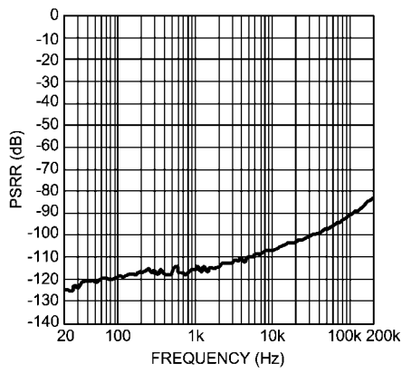
PSRR+ vs Frequency V_{CC} = 17V, V_{EE} = -17V R_L = 2k\Omega, f = 200kHz, V_{RIPPLE} = 200mVpp
