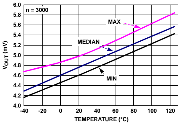
FIGURE 35. ISL28271 V_{OUT} LOW vs TEMPERATURE, R_L = 100k , V_+ = V_- = \pm 2.5V
