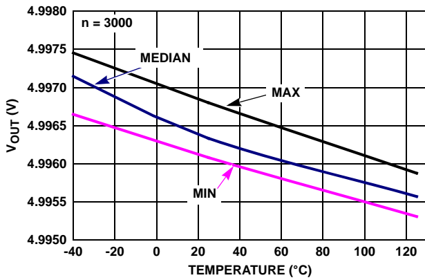
FIGURE 31. ISL28271 V_{OUT} HIGH vs TEMPERATURE, R_L = 100k , V_+ = V_- = \pm 2.5V
