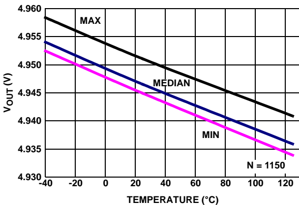
FIGURE 34. V_{OUT \text{ HIGH}} vs TEMPERATURE V_+ = 5V , V_- = 0V , V_{CM} = 2.5V , R_L = 1k
