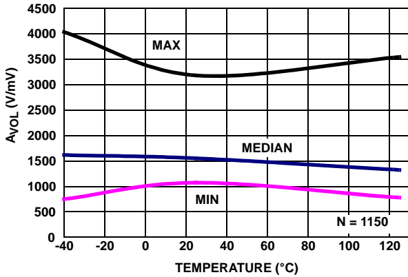
FIGURE 32. AVOL vs TEMPERATURE V_+ = 5V , V_- = 0V , V_{CM} = 2.5V , R_L = \text{Open}
