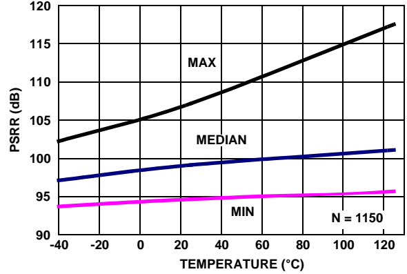
FIGURE 31. PSRR vs TEMPERATURE V_+ = 5V , V_- = 0V , V_{CM} = 2.5V , R_L = \text{Open}
