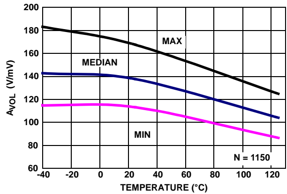
FIGURE 33. AVOL vs TEMPERATURE V_+ = 5V , V_- = 0V , V_{CM} = 2.5V , R_L = 1k
