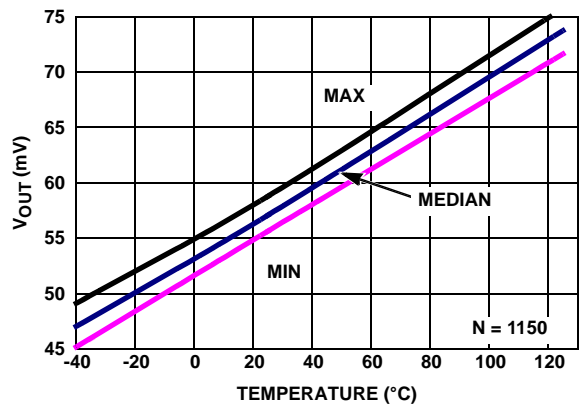
FIGURE 35. V_{OUT \text{ LOW}} vs TEMPERATURE V_+ = 5V , V_- = 0V , V_{CM} = 2.5V , R_L = 1k
