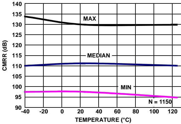
FIGURE 30. CMRR vs TEMPERATURE V_{CM} = +2.5V TO -2.5V , V_+ = 5V , V_- = 0V , R_L = \text{Open}
