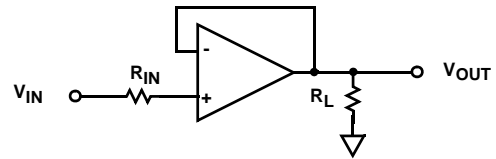
FIGURE 36. INPUT CURRENT LIMITING
