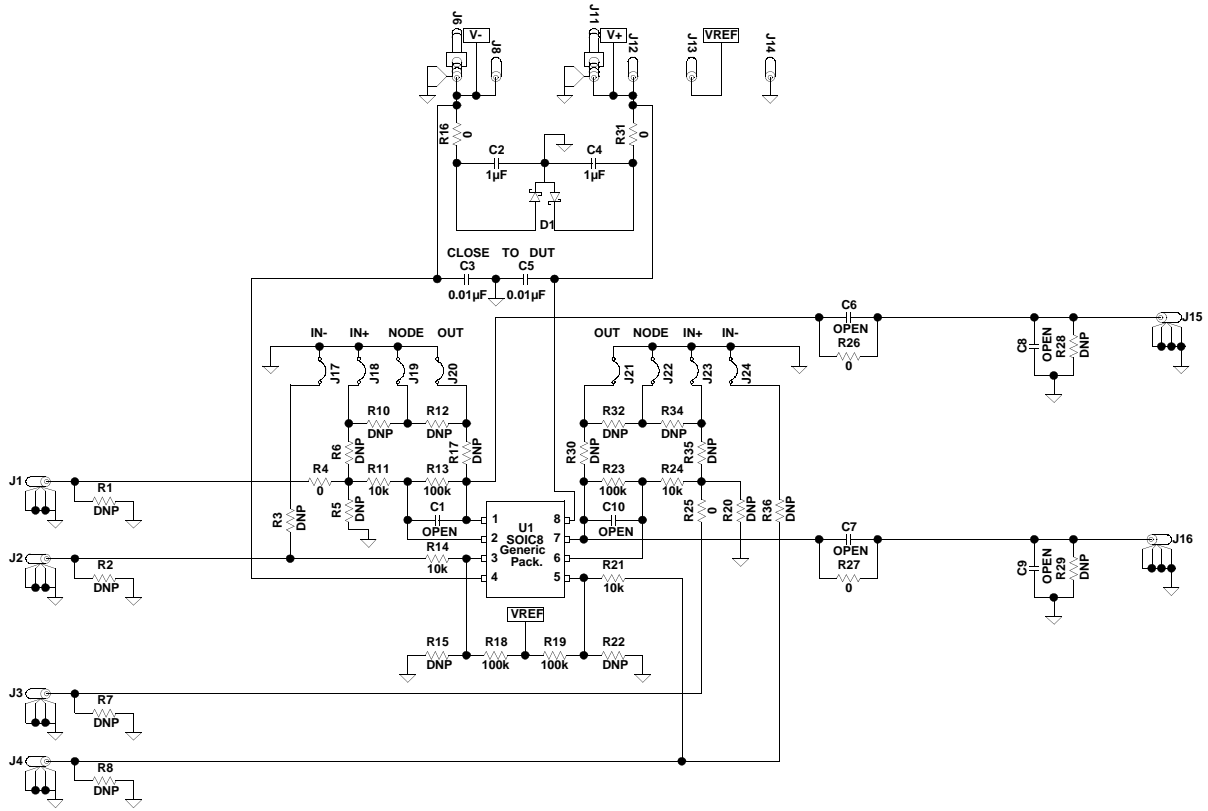
FIGURE 6. ISL282X7SOICEVAL2Z SCHEMATIC DIAGRAM
