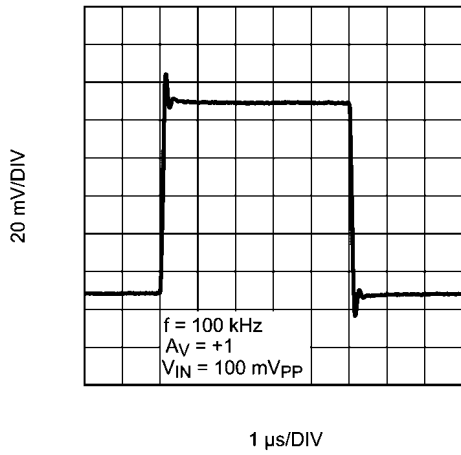
Small Signal Step Response with Gain = 1
