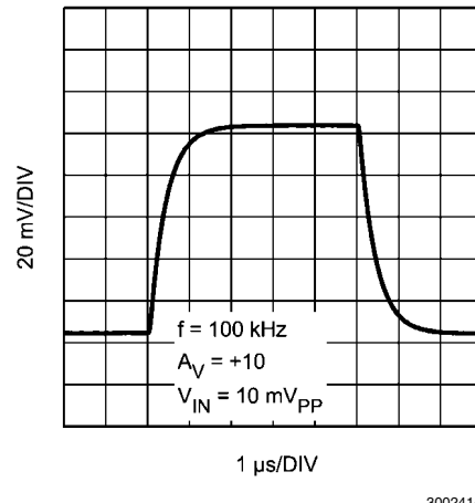
Small Signal Step Response with Gain = 10
