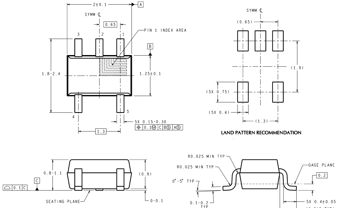
5-Pin SC70 NS Package Number MAA05A
