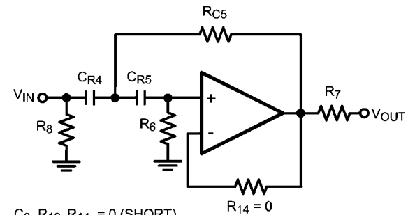
FIGURE 8. Sallen-Key High-Pass Filter
