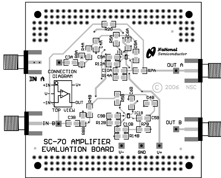
FIGURE 18. 551012922-001 Top Layout
