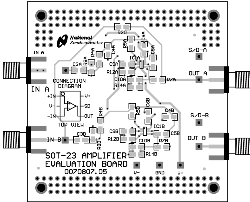
FIGURE 15. 551012875-001 Top Layout
