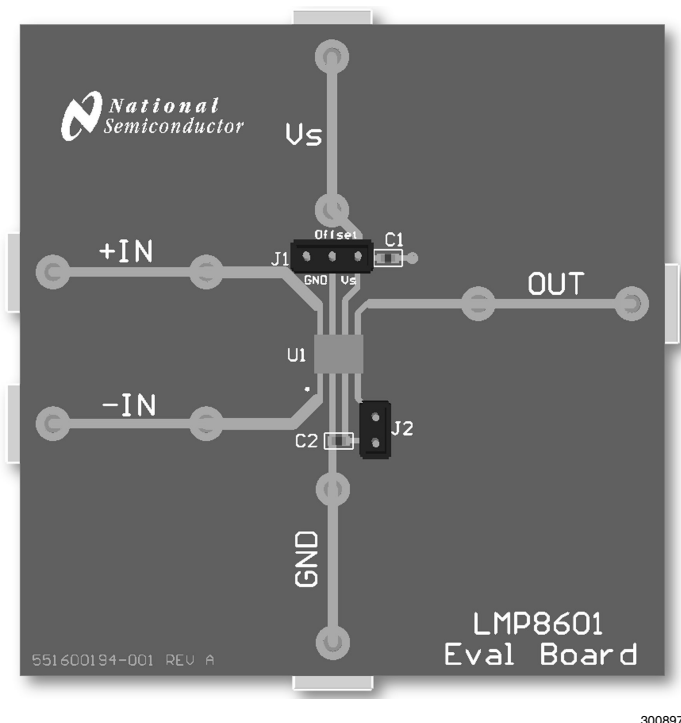
FIGURE 1. The LMP8601 Evaluation Board
