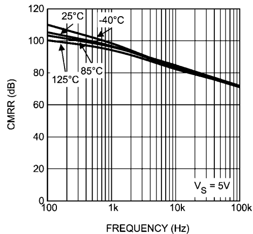
CMRR vs. Frequency at V_S = 5\text{V}
