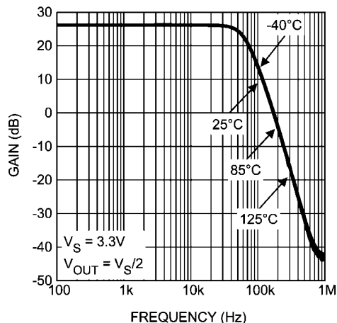
Gain vs. Frequency at V_S = 3.3\text{V}
