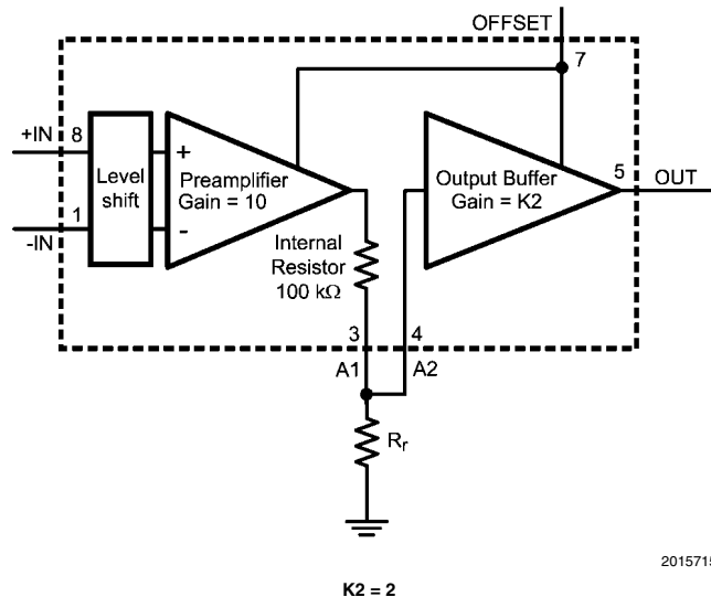
FIGURE 3. Reduce Gain
