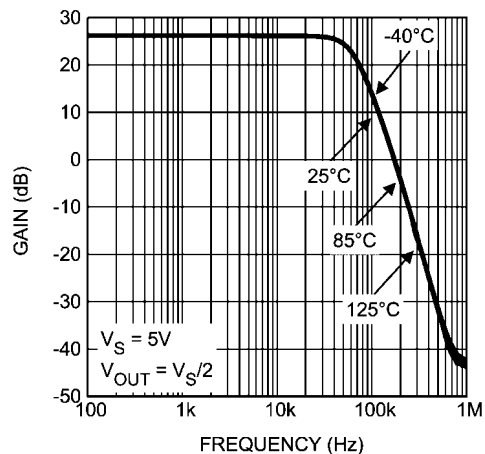
Gain vs. Frequency at V_S = 5\text{V}
