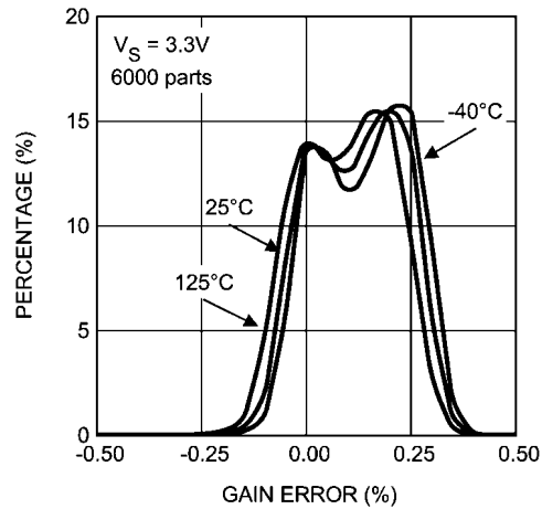
Gain error Distribution at V_S = 3.3V
