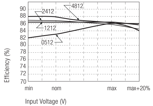
Efficiency VS Input Voltage
