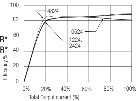
Efficiency / Load
