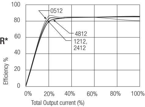
Efficiency / Load
