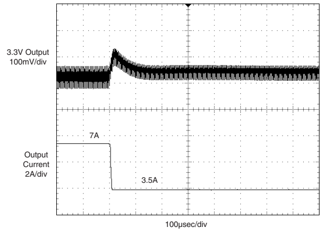
3.3V Output Full-Load to Half-Load Transient Response (VIN = nominal, 5V @ 600mA, external 1µF output capacitors.)
