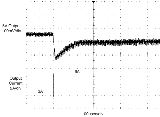
5V Output Half-Load to Full-Load Transient Response (VIN = nominal, 3.3V @ 700mA, external 1µF output capacitors.)
