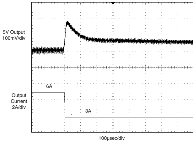
5V Output Full-Load to Half-Load Transient Response (VIN = nominal, 3.3V @ 700mA, external 1µF output capacitors.)
