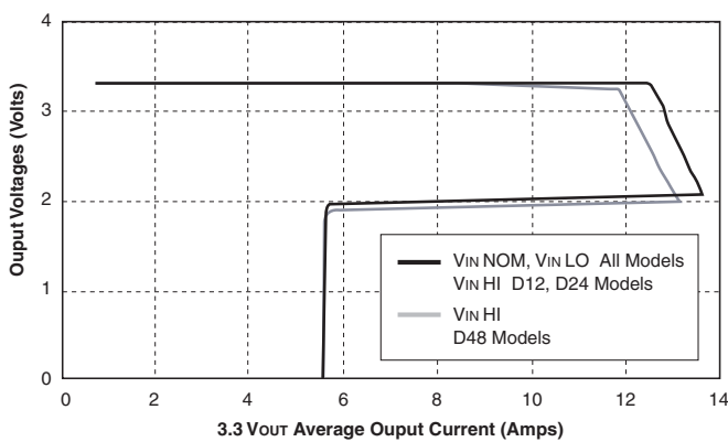
Figure 2a. Current Limiting Characteristics for 3.3V Output
