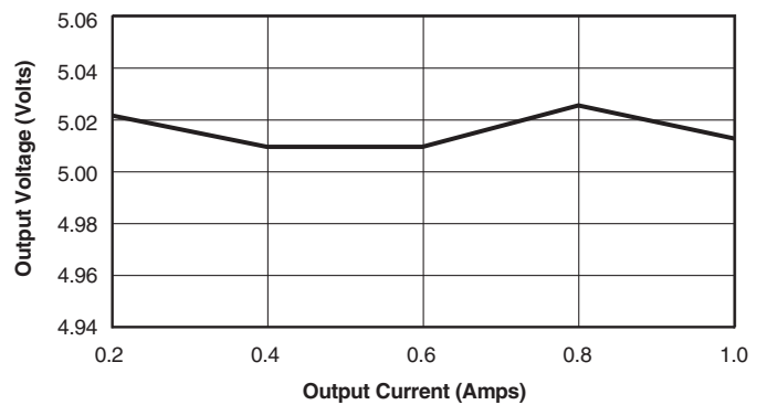
Output Voltage vs. Output Load
