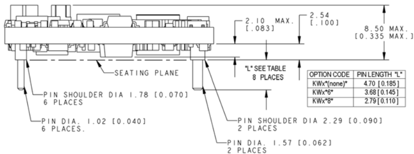
Side View
