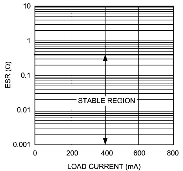
FIGURE 1. Stable Region For Output Capacitor ESR
