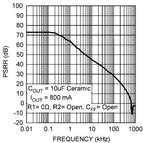
PSRR, I_{OUT} = 800 \text{ mA} V_{OUT} = V_{ADJ} , C_{OUT} = 10 \mu F Ceramic
