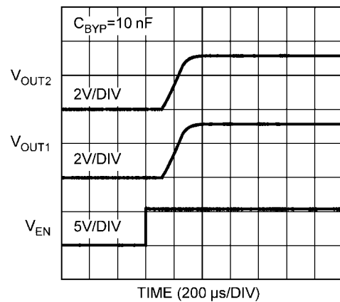
Enable Start-up Time, C_{BYF}=10\text{nF}
