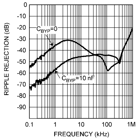
Power Supply Rejection Ratio, LDO1
