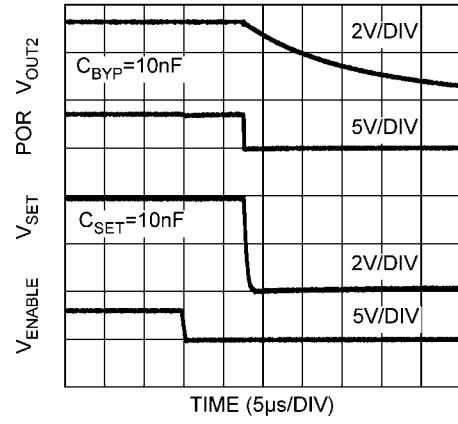
Power-on-Reset Shutdown Operation
