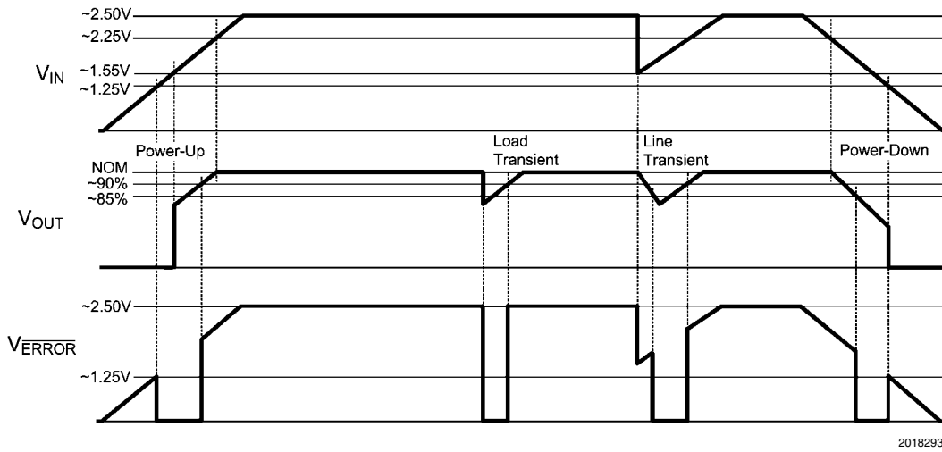
FIGURE 2. \overline{V_{ERROR}} Flag Operation, biased from V_{IN}
