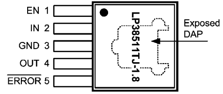
Top View TO-263 THIN 5 Pin Package
