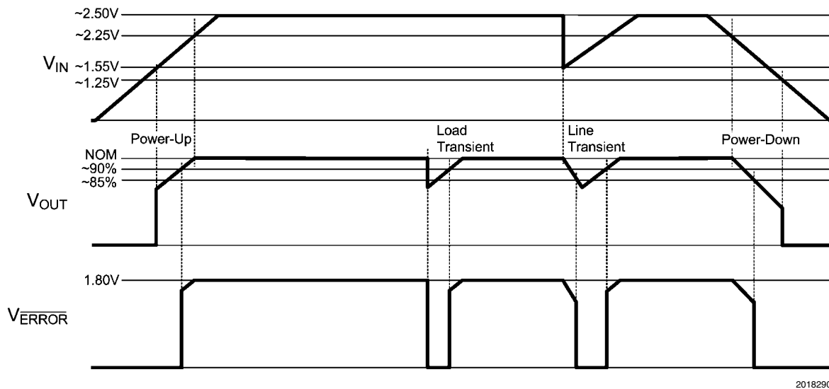
FIGURE 1. \overline{\text{ERROR}} Flag Operation, see Typical Application
