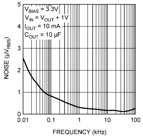
Output Noise
