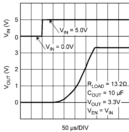
V OUT vs V IN , Power-Up
