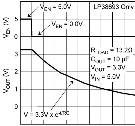
V OUT vs V EN , OFF (LP38693 Only)
