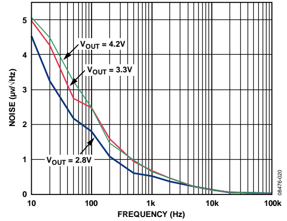
Figure 22. Output Noise Spectrum, V_{IN} = 5V
