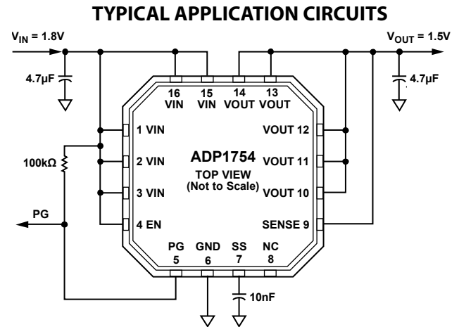
Figure 1. ADP1754 with Fixed Output Voltage, 1.5 V
