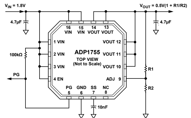
Figure 2. ADP1755 with Adjustable Output Voltage, 0.75 V to 3.0 V
