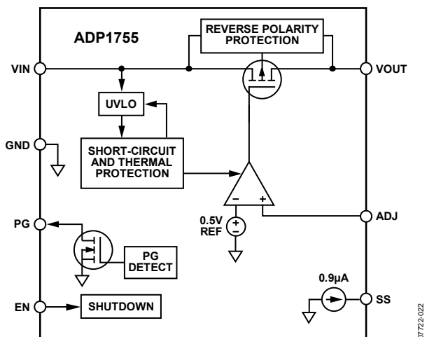
Figure 25. ADP1755 Internal Block Diagram
