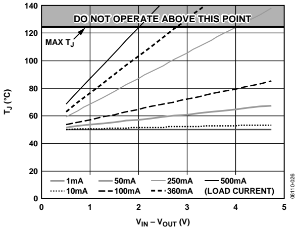
Figure 38. 0.70 mm 2 of PCB Copper, T A = 50°C
