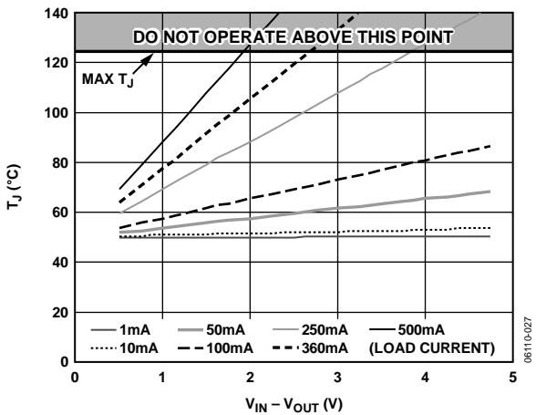
Figure 39. 0.30 mm 2 of PCB Copper, T A = 50°C
