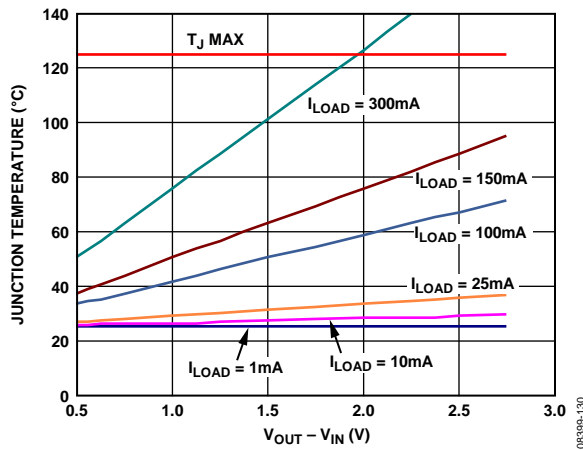
Figure 36. Junction Temperature vs. Power Dissipation, 0 mm 2 of PCB Copper, T A = 25°C
