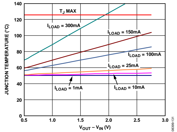
Figure 37. Junction Temperature vs. Power Dissipation, 500 mm 2 of PCB Copper, T A = 50°C
