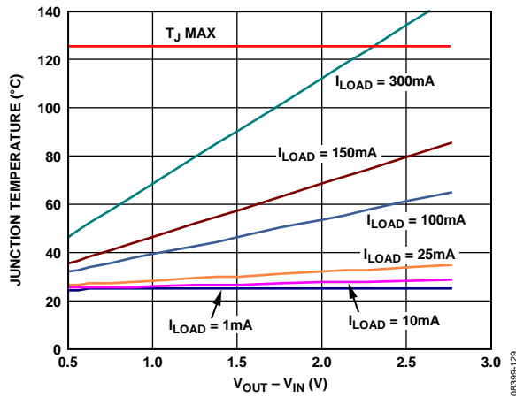
Figure 35. Junction Temperature vs. Power Dissipation, 100 mm 2 of PCB Copper, T A = 25°C
