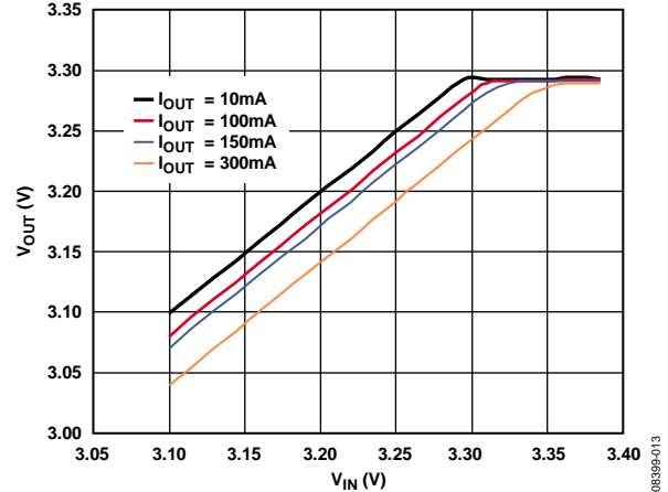
Figure 14. Output Voltage vs. Input Voltage (in Dropout)
