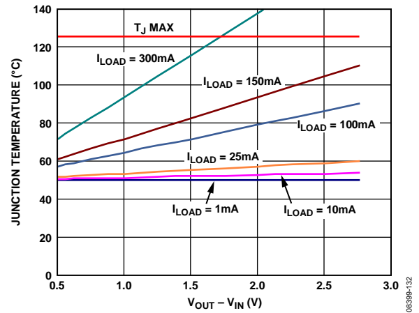
Figure 38. Junction Temperature vs. Power Dissipation, 100 mm 2 of PCB Copper, T A = 50°C
