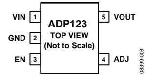
Figure 4. ADP123 Adjustable Output Pin Configuration
