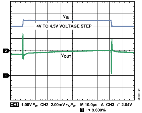
Figure 25. Line Transient Response, Load Current = 300 mA
