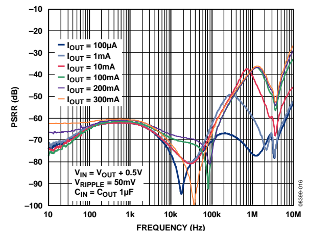
Figure 16. Power Supply Rejection Ratio vs. Frequency, V_{OUT} = 3.3V , V_{IN} = 3.8V
