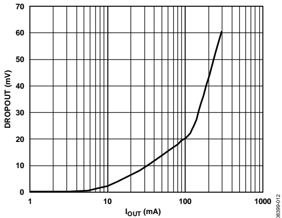
Figure 12. Dropout Voltage vs. Load Current
