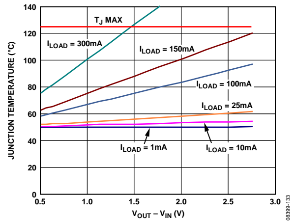
Figure 39. Junction Temperature vs. Power Dissipation, 0 mm 2 of PCB Copper, T A = 50°C
