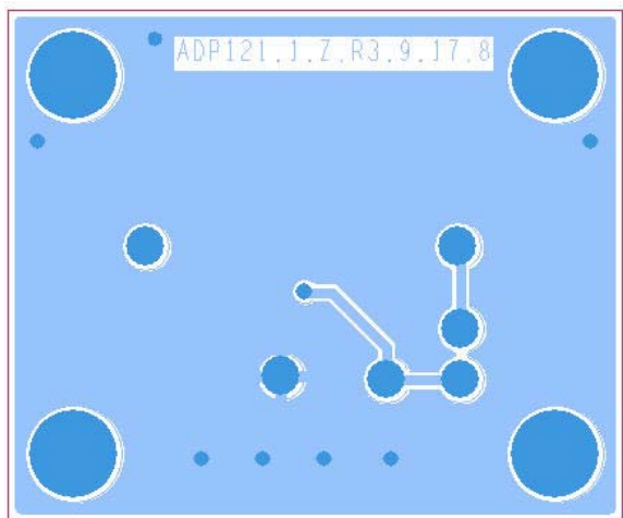
Figure 50. Example of WLCSP PCB Layout—Bottom Side
