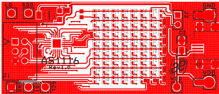
Figure 4: Top Layer
