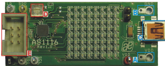
Figure 1: Board Description - Connectors
