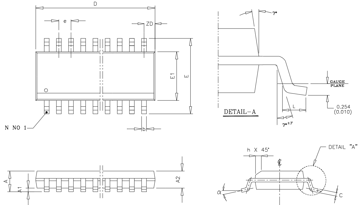
Figure 21. QSOP-24 Package
