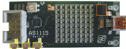
Figure 2: Board Description – Switches
