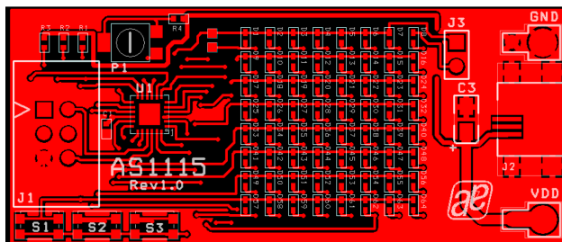
Figure 4: Top Layer
