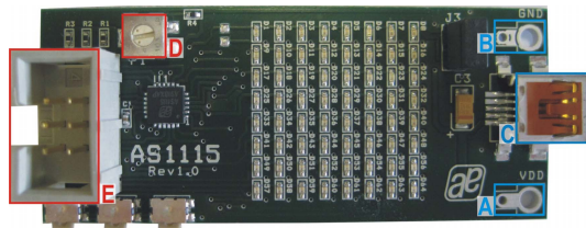
Figure 1: Board Description - Connectors
