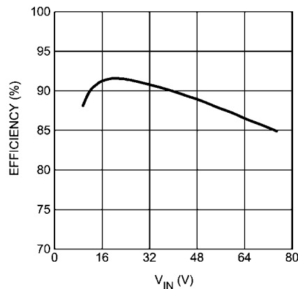
EFFICIENCY WITH 9 SERIES LEDS AT 1A
