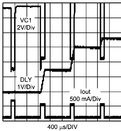
FIGURE 5. Fault Delay Waveforms (one LED open)
