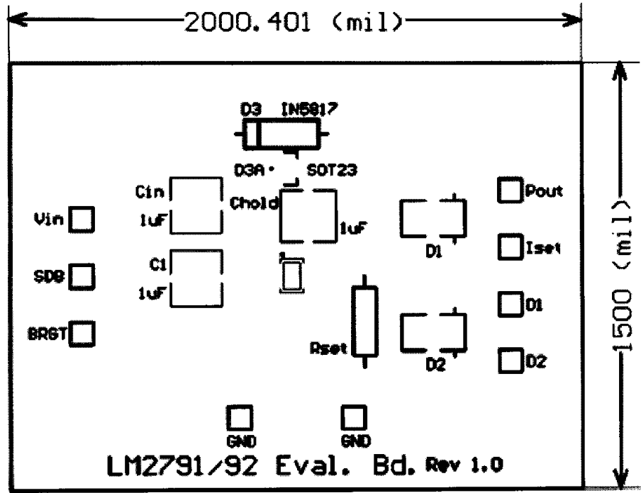
FIGURE 1. Silkscreen
