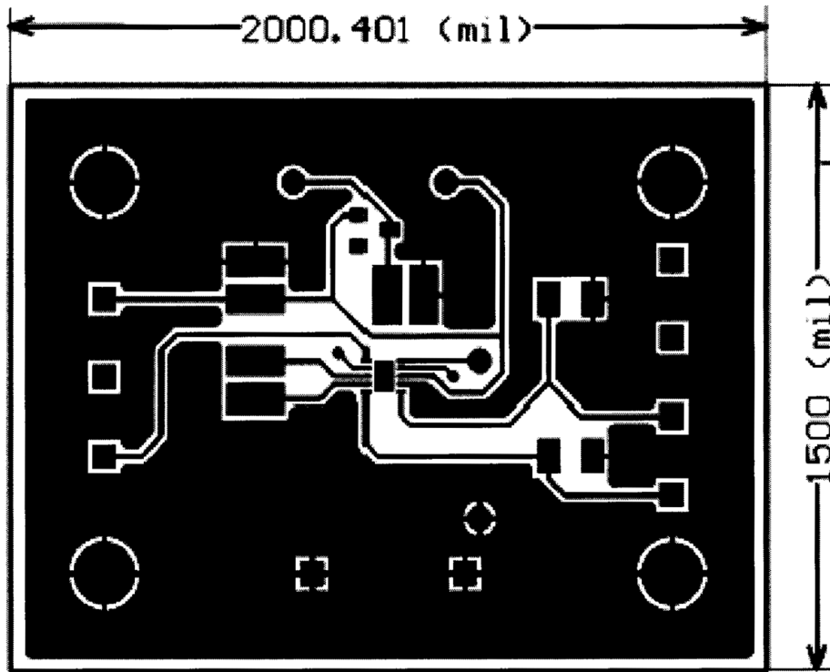
FIGURE 2. PCB Layout
