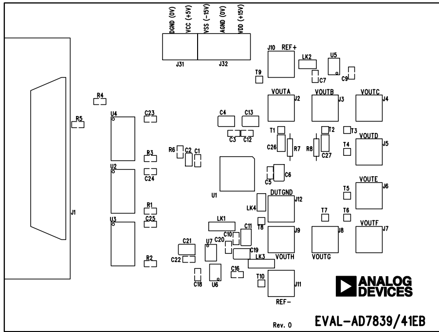
AD7839 EVALUATION BOARD - COMPONENT SIDE VIEW
