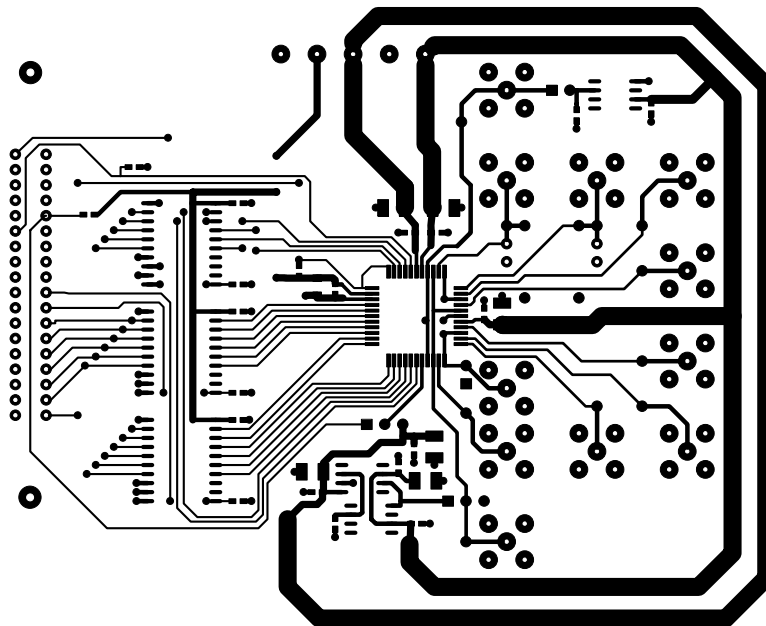
AD7839 EVALUATION BOARD - COMPONENT SIDE VIEW
