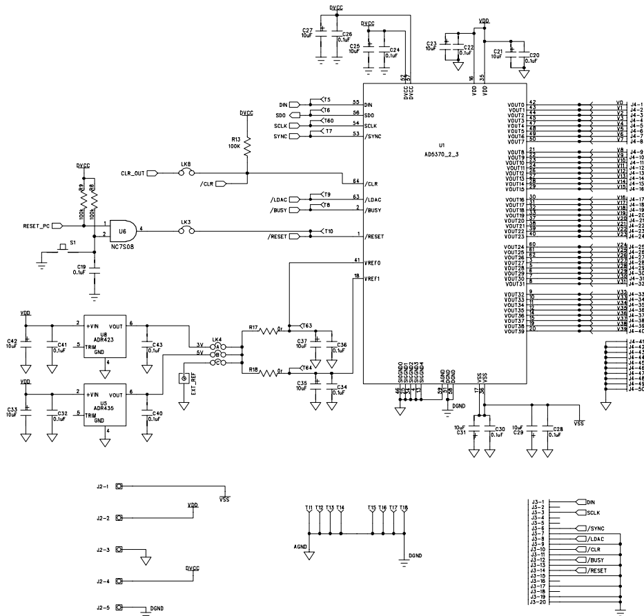
Figure 6. AD537x Schematic (1 of 2)
