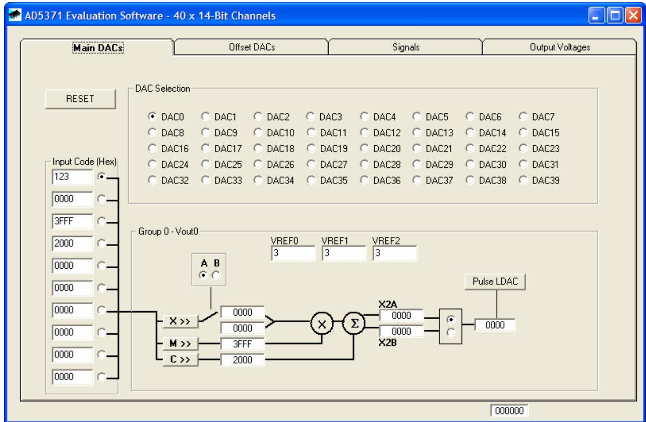
Figure 2. AD537x Tab 1 Software Screenshot
