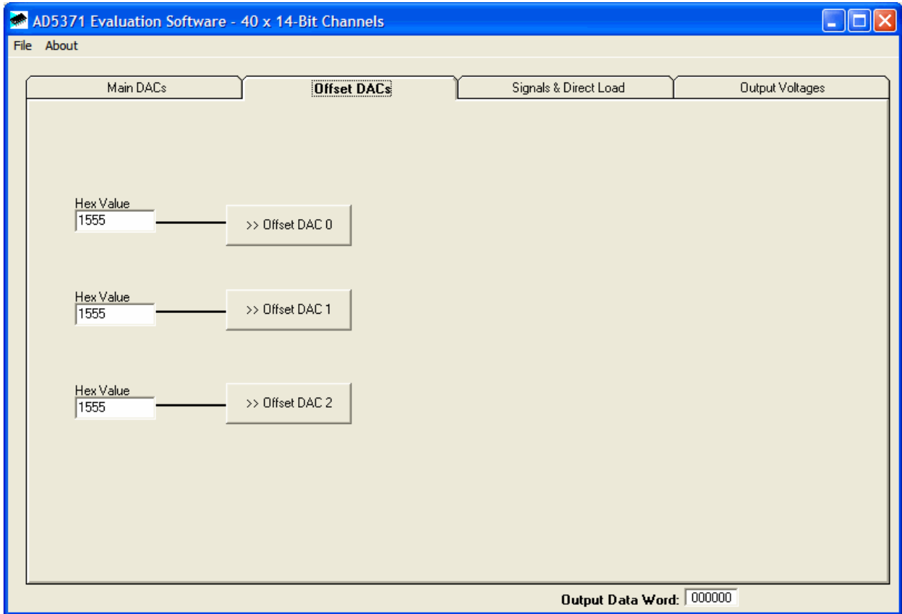
Figure 3. AD537x Tab 2 Software Screenshot
