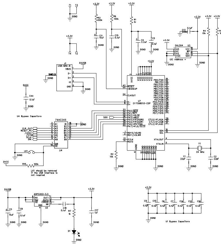
Figure 7. AD537x Schematic (2 of 2)
