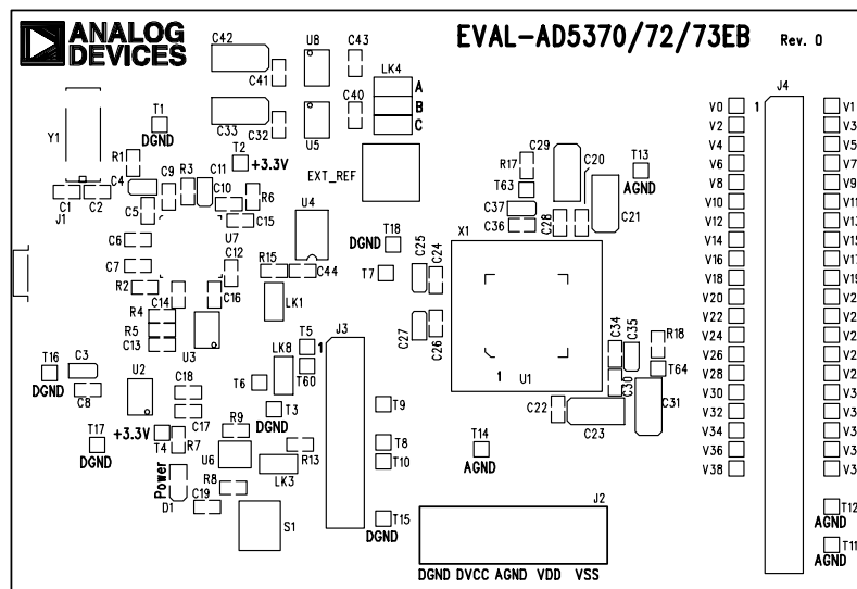
Eval-AD5370/72/73EB Rev. 0 (Component Side View)
