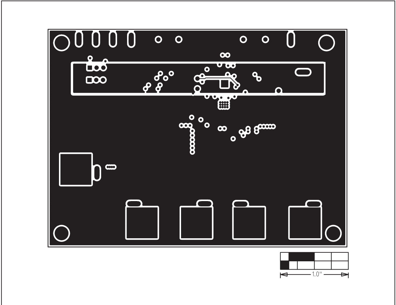
Figure 5. MAX15023 EV Kit PCB Layout—Inner Trace Layer 3
