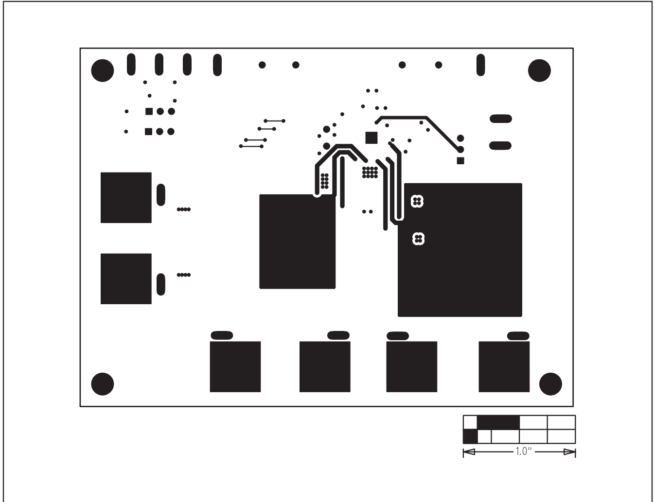
Figure 6. MAX15023 EV Kit PCB Layout—Solder Side
