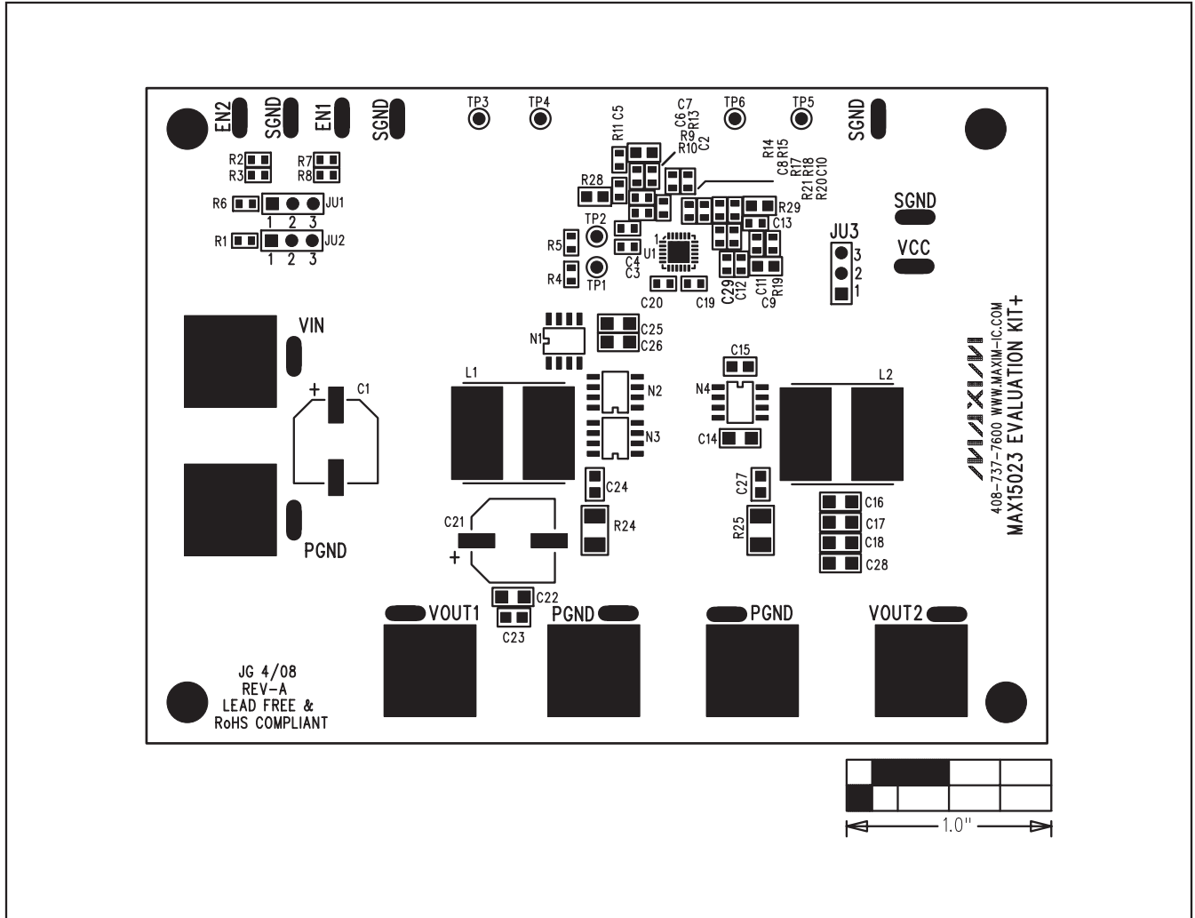
Figure 2. MAX15023 EV Kit Component Placement Guide—Component Side
