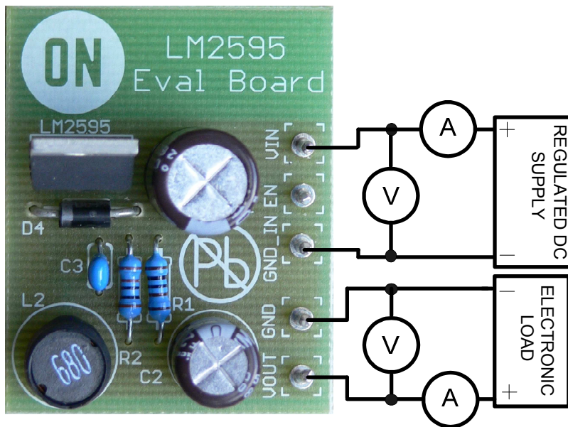
Figure 1: Test Setup
