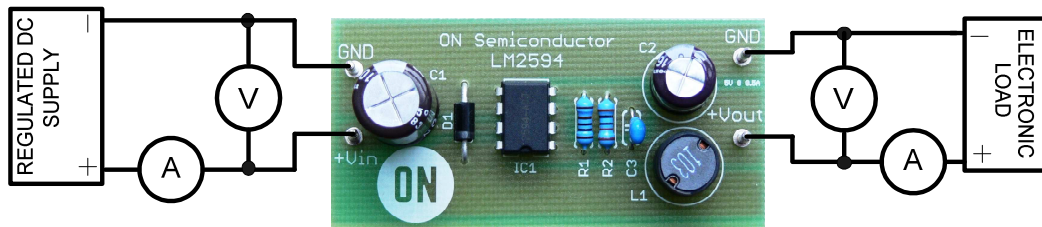
Figure 1: Test Setup
