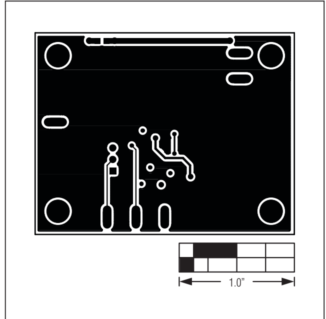
Figure 6. MAX15041 EV Kit PCB Layout—Solder Side
