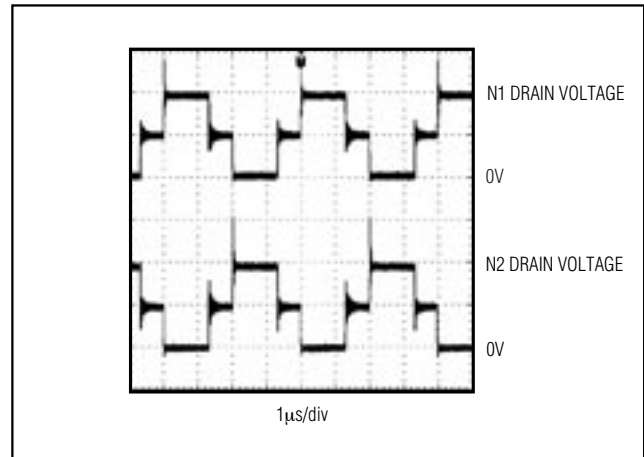
Figure 1. MOSFETs N1 and N2 Drain-Source Voltage Waveforms (50V per Division, 1µs per Division)
