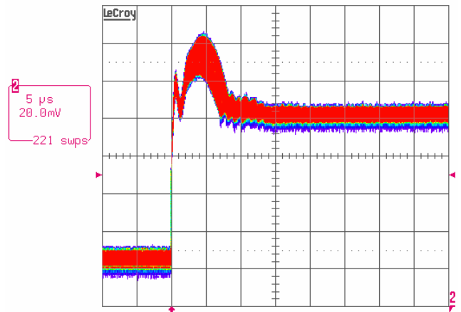
FIGURE 43. LOAD TRANSIENT RESPONSE WITH OVERSHOOT REDUCTION FUNCTION DISABLED, V_{IN} = 12V , SV CLARKSFIELD CPU TEST CONDITION: VID = 0.95V, I_O = 12A/51A , di/dt = "FASTEST", LL = 1.9mΩ
