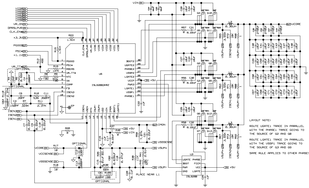
FIGURE 27. 3-PHASE REFERENCE DESIGN
