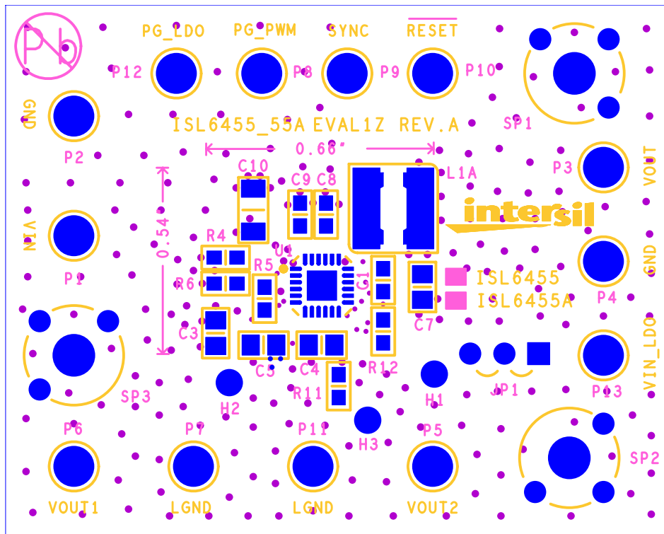
FIGURE 1. TOP COMPONENTS
