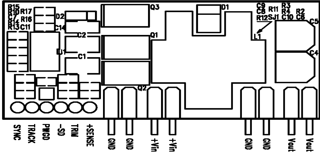
FIGURE 12. Top Silkscreen
