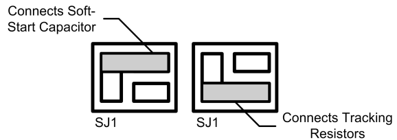
FIGURE 1. Soft-Start and Tracking Jumper
