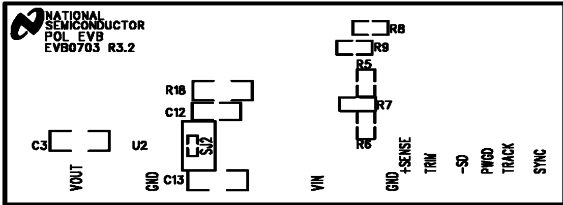
FIGURE 14. Bottom Silkscreen
