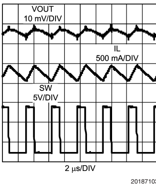
FIGURE 3. PWM Waveforms ( I_{OUT} = 1A )
