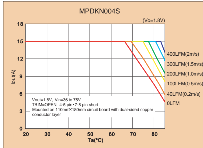
Temperature Derating Characteristic
