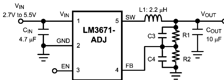
FIGURE 2. Adjustable Output Voltage — Typical Application Circuit
