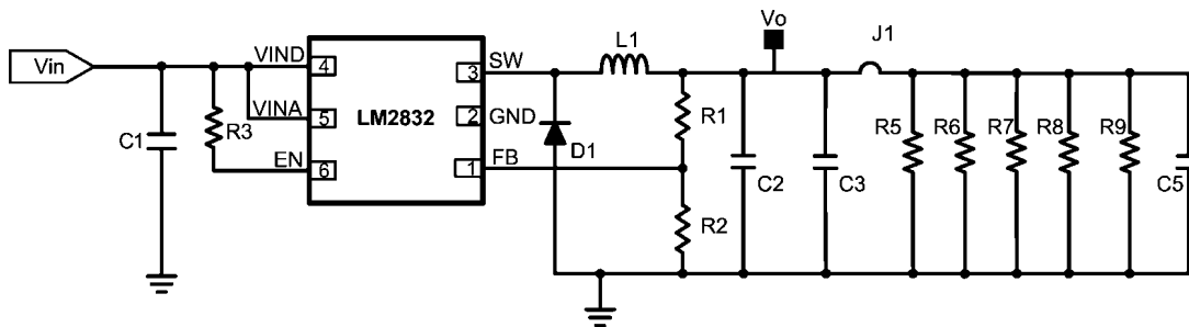
LM2832Z 6-Pin LLP Demo Board Schematic
